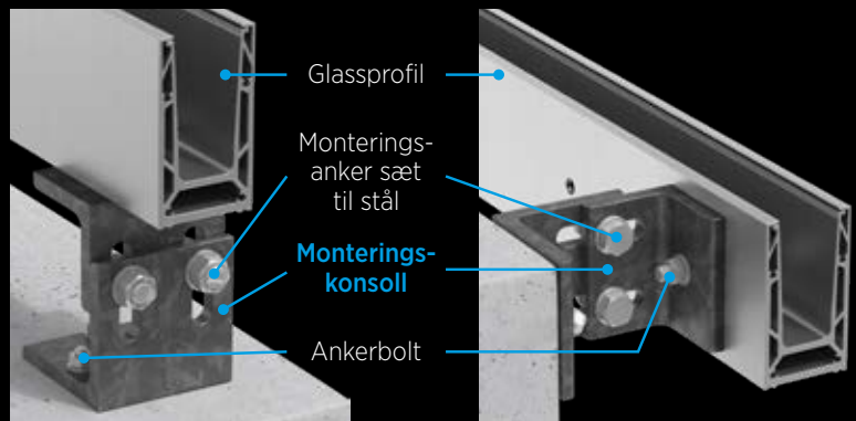
Toppmontering
